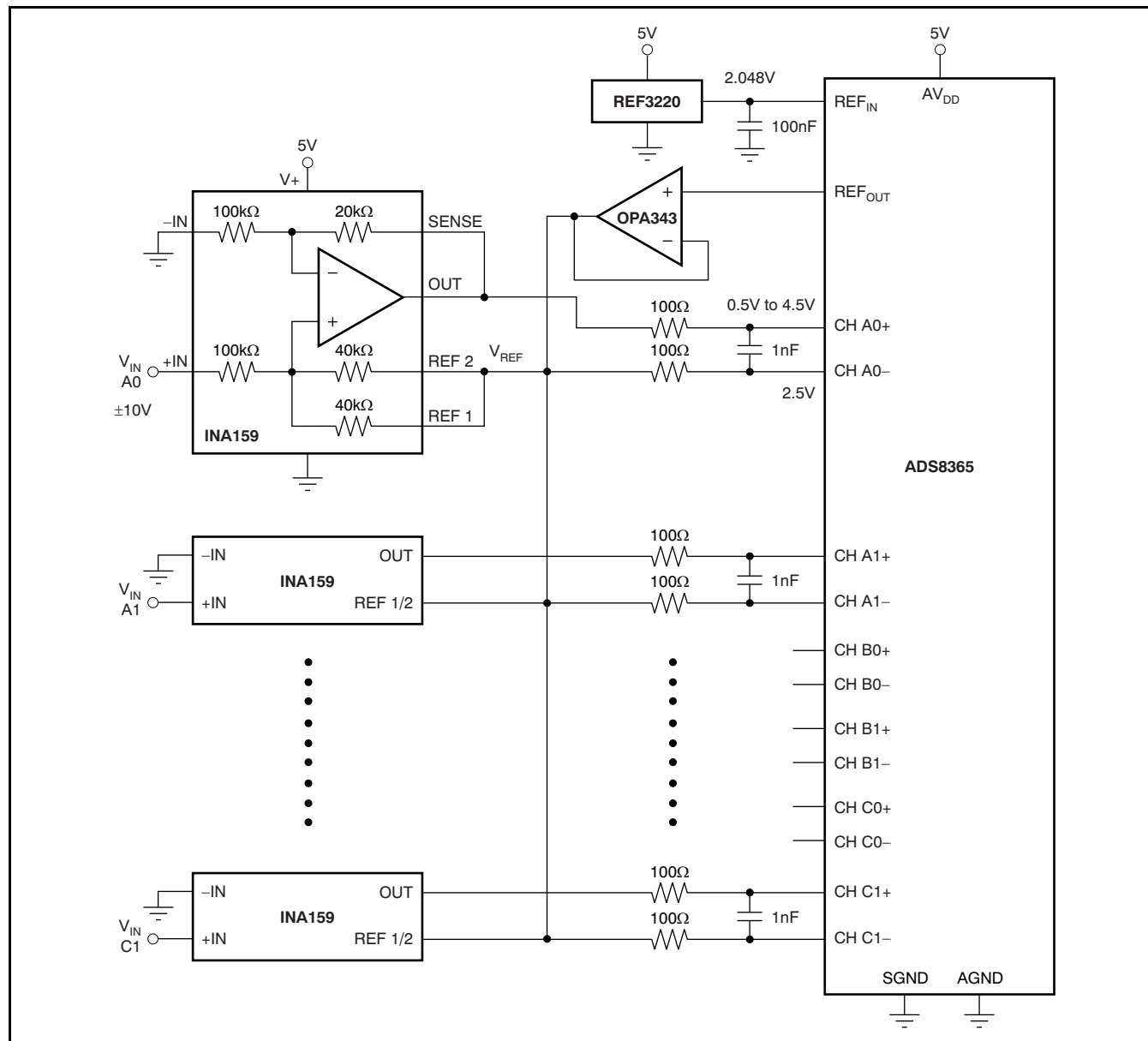
Figure 33. \pm 10\text{V} Input Range By Using the INA159
