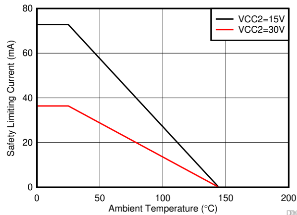
图 6-1. Thermal Derating Curve for Limiting Current per VDE for D Package
